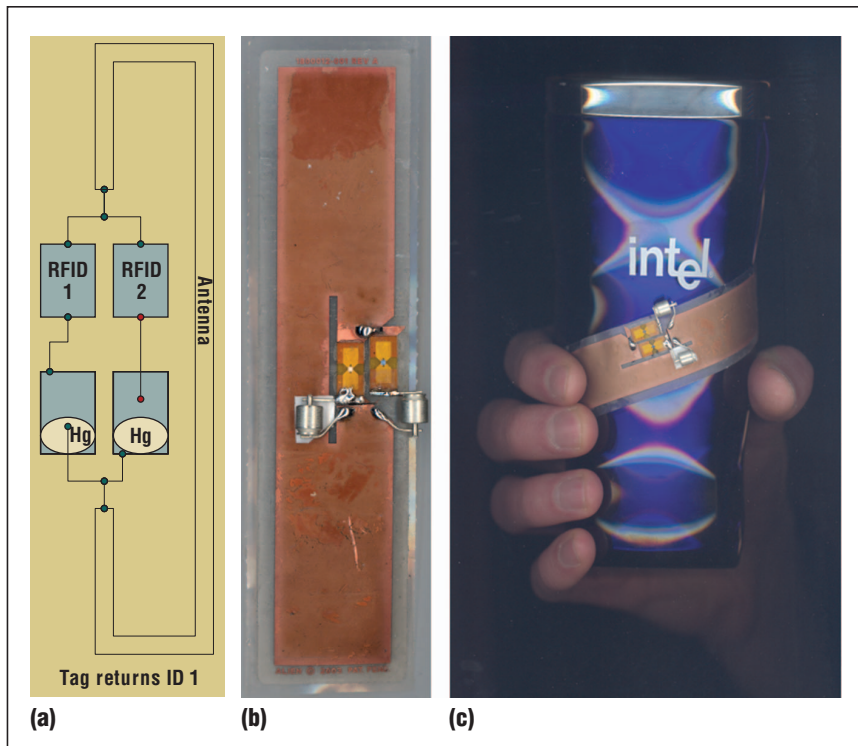
Figure 1. a-Wisp serial-switch configuration: (a) schematic, (b) photograph, (c) deployment on a coffee cup.
