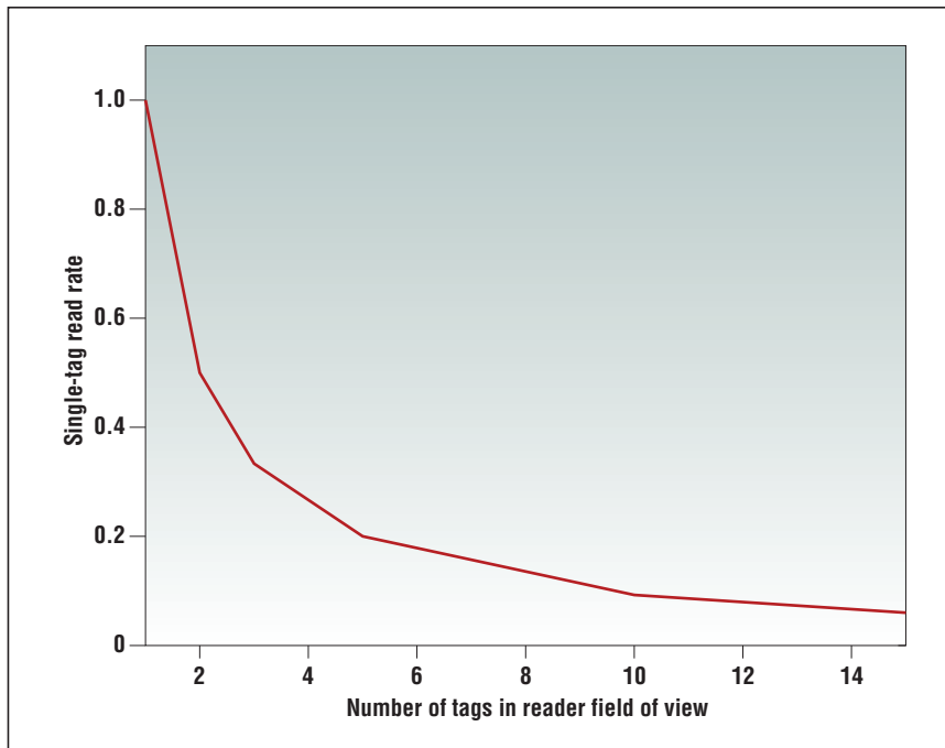
Figure 3. The effects of a worst-case dense tag deployment. The fraction of deployed tags that the reader can read is inversely proportional to the number of tags deployed. The tags are spaced uniformly in a 0.6-meter-wide paper envelope, read over 30-second windows, at a 0.9-meter range.
